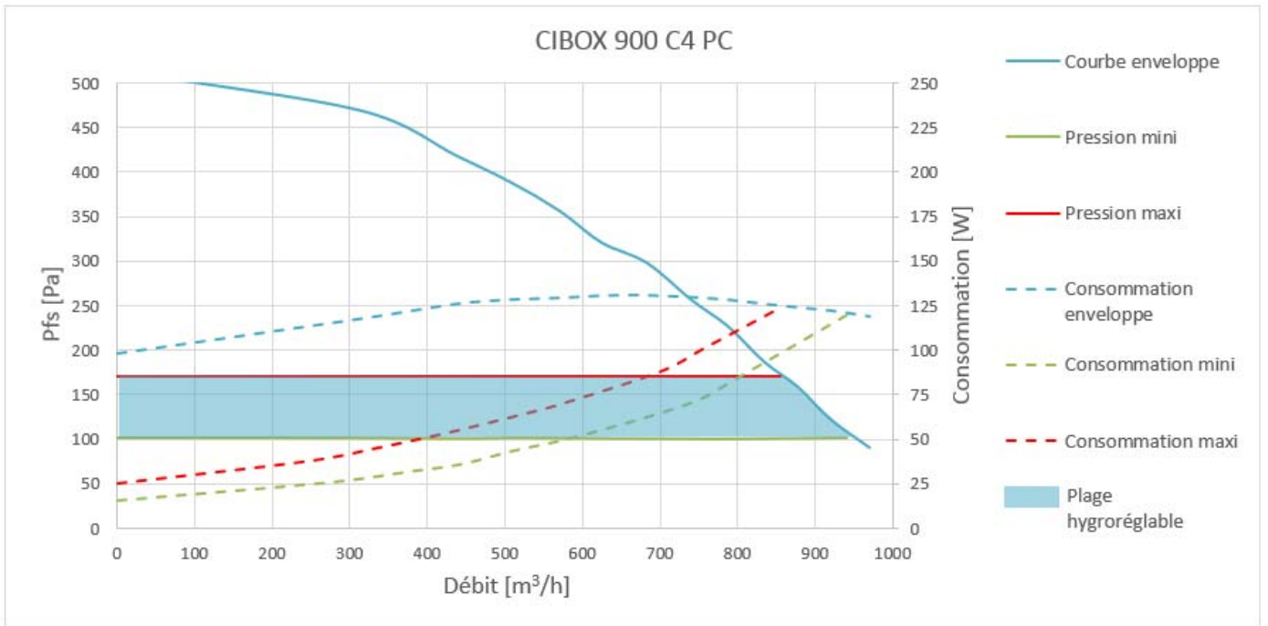
Figure 3 – CIBOX 900 C4 PC
