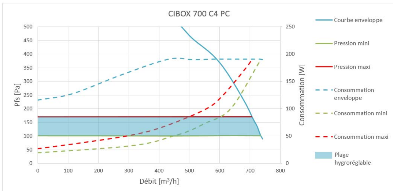
Figure 2 – CIBOX 700 C4 PC
