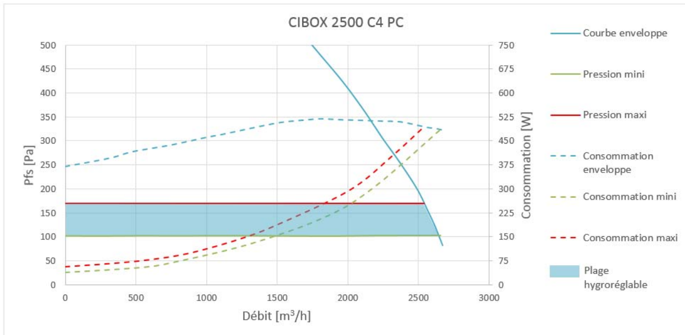
Figure 5 – CIBOX 2500 C4 PC
