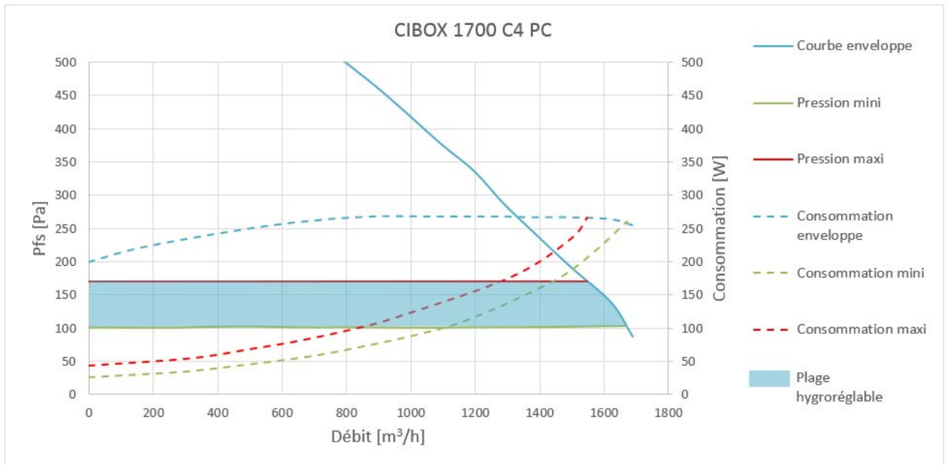
Figure 4 – CIBOX 1700 C4 PC
