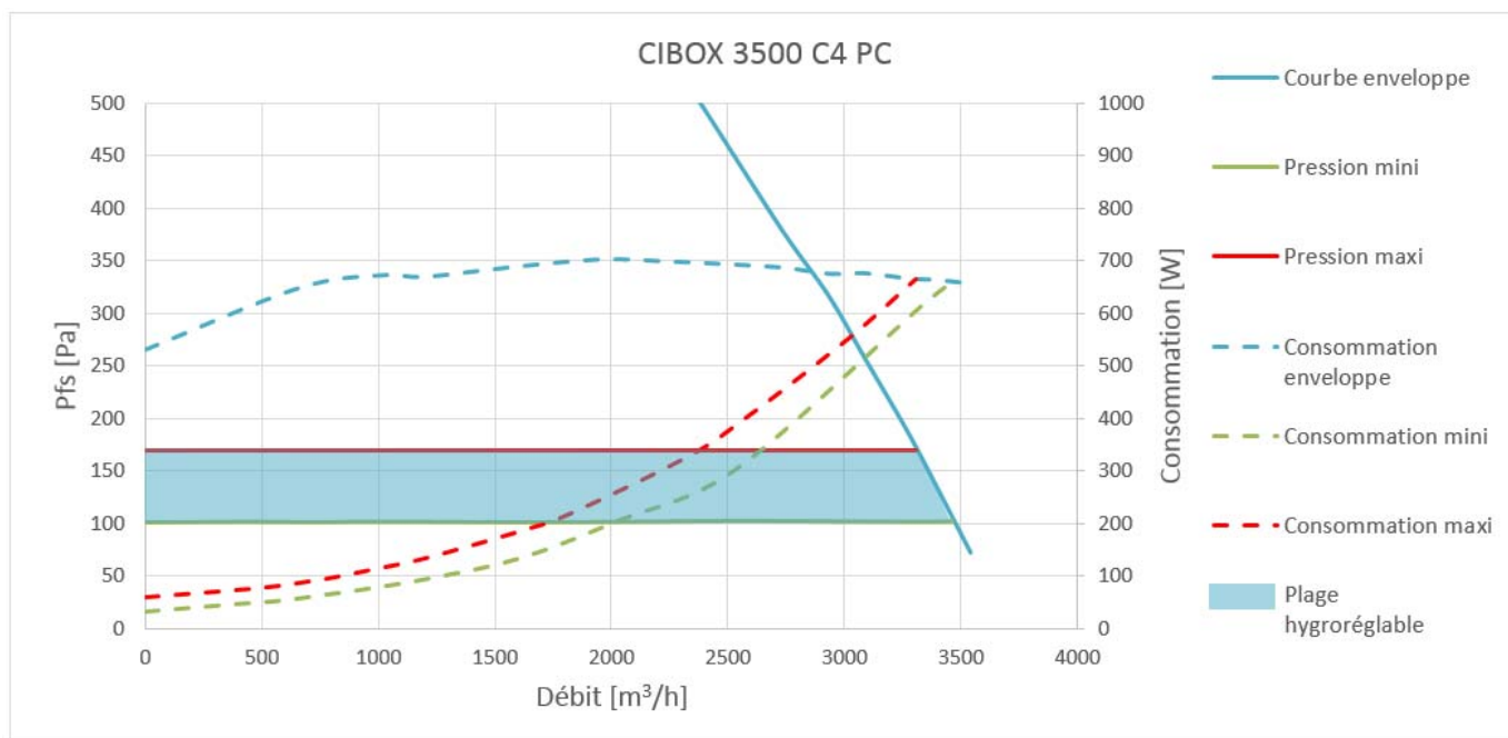
Figure 6 – CIBOX 3500 C4 PC
